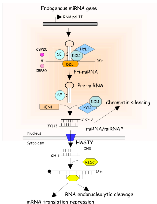
Figure 7: Biogenesis and activity of miRNAs in Arabidopsis (Brodersen et al. , 2006; Voinnet, 2009)
