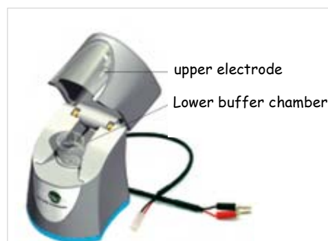
Figure 7: FlashPAGE fractionator
