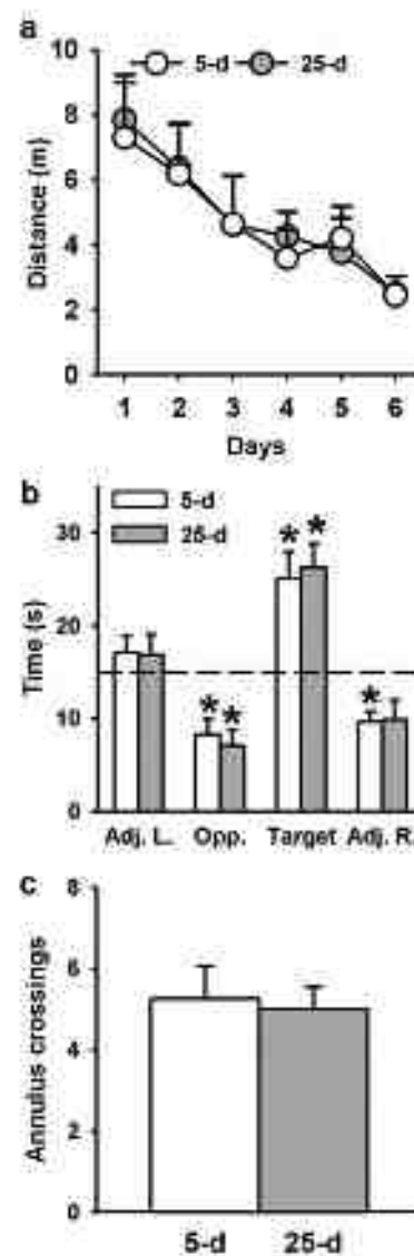
Figure 1. Spatial memory performance during acquisition and probe trial in the water-maze task with a hidden platform. a , Average distance ( \pm SEM) to reach the platform during water-maze training in rats subsequently tested for recent (5 d, n = 11 ) or remote (25 d, n = 7 ) memory retrieval. All rats were subjected to four daily trials over 6 consecutive days. There were no significant differences between the two delay groups. b , c , Mean performance ( \pm SEM) during probe trials performed 5 d (recent memory) or 25 d (remote memory) after the end of training. Probe trial performance is expressed as the time (in seconds) spent in the four virtual quadrants of the pool (0) and the number ( \pm SEM) of crossings over the target annulus. The dotted line is chance level (chance level, 50 trials). *Significantly different from chance (i.e., 15 s), p < 0.05 . All rats remembered the platform location and concentrated their searches in the target quadrant where the platform was located during task acquisition. d , e , Spatially-athetic delay 25 d, 25 d postacquisition delay. Adj. L., quadrant at the left of the target quadrant; Opp., quadrant opposite to the target quadrant; Adj. R., quadrant at the right of the target quadrant; Target, quadrant where the platform was located during training.
