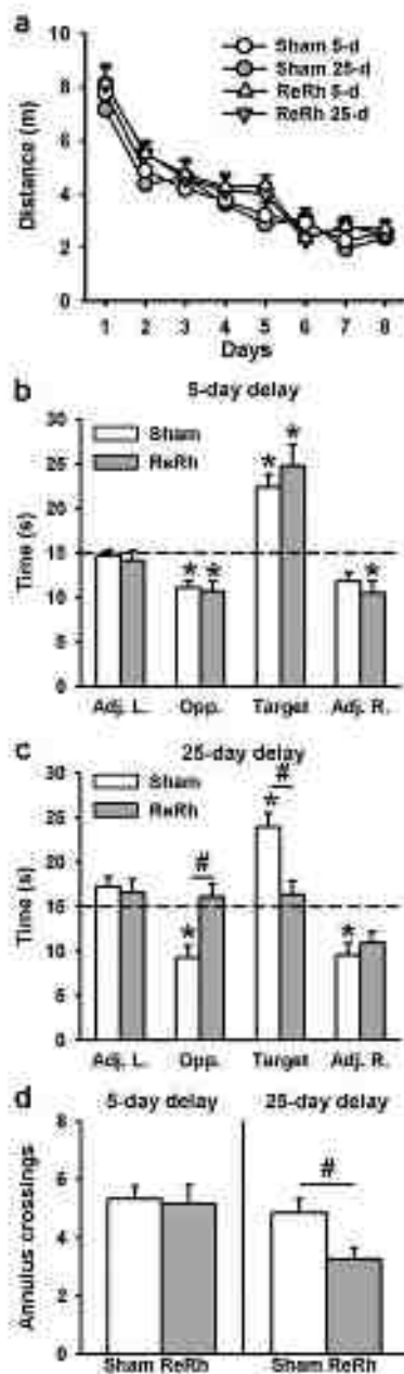
Figure 4. Effects of a pre-acquisition ReRh lesion on spatial memory performance during acquisition and retrieval in the hidden version of the water-maze task. a , Average distance ( n = 50 ) to reach the platform during water-maze acquisition in the rats who were tested for recent (5 d) or remote (25 d) memory in Sham and ReRh groups. Rats were subjected to four daily training trials per consecutive days. There were no significant differences between the four groups. b–d , Mean performance ( n = 50 ) during recent and remote memory probe trials, expressed as the time (in seconds) spent in the four arena quadrants of the pool, c , and the number ( n = 50 ) of crossings over the target area ( d ) at the 5 day (left) and 25 day (right) postacquisition delay. The dashed line represents chance level ( n = 3 s; Statistics: p < 0.05 , versus Sham; significantly different from chance, p < 0.05 , than intervention of the platform location and concentrated their searches in the target quadrant where the platform was located over training. In contrast, ReRh lesion rats, both at the 5 day delay, even though they kept exploring the pool, the number of crossings at 5 day delay ( n_{\text{Sham}} = 5.5 , n_{\text{ReRh}} = 11 ; 25 day delay, n_{\text{Sham}} = 5.0 , n_{\text{ReRh}} = 3.5 ) at postacquisition delay. 25 d, 25 d postacquisition delay; Adj. L., quadrant at the left of the target quadrant; Opp., quadrant opposite to the
