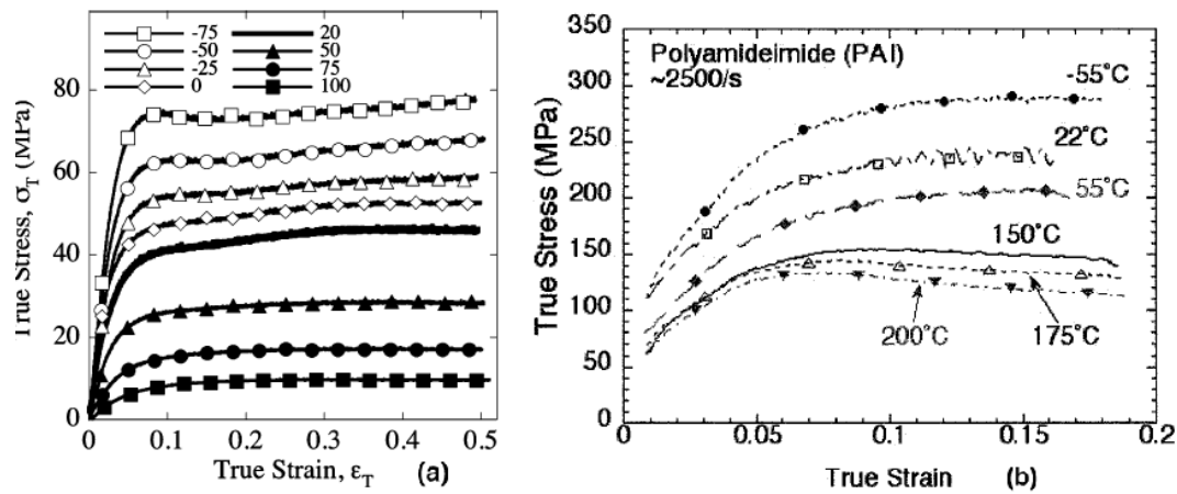
Figure 1-17: Mechanical response of (a) HDPE and (b) PAI as a function of temperature under strain rate 10^{-2} \text{ s}^{-1} , 2500 \text{ s}^{-1} , respectively [40].
