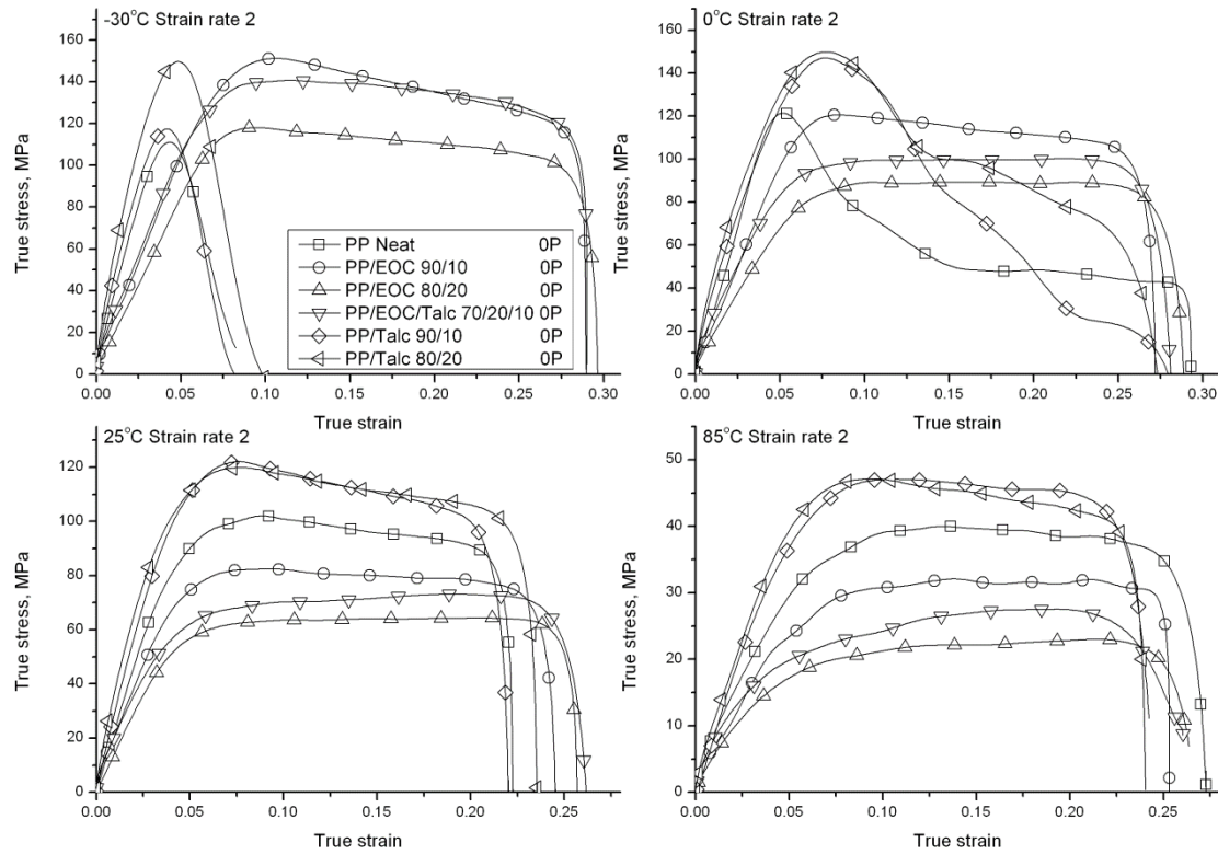
Figure 3-2: True stress - true strain curves in compression of non-recycled neat PP and its composites at different temperatures and under strain rate 2 (strain-rate-2 = 1276 \text{ s}^{-1} ).
