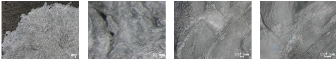
Figure 3-8: OM images of non-recycled and recycled neat PP and PP-based composites after the dynamic compressive test at -30 °C and under strain rate 4.
