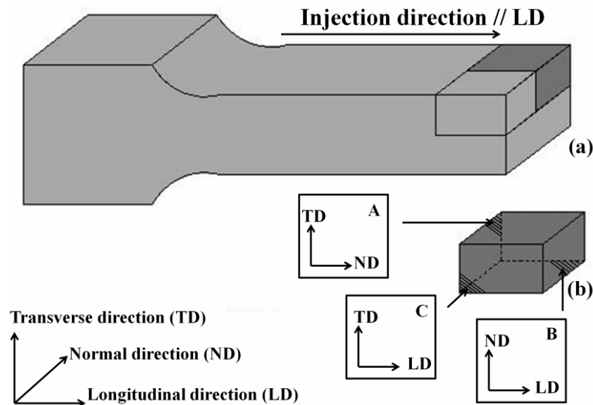
Figure 2-2: Sample preparation for the WAXS and SEM observation: (a) a half of slice was cut from the center of the sample, (b) definition of the planes of interest.
