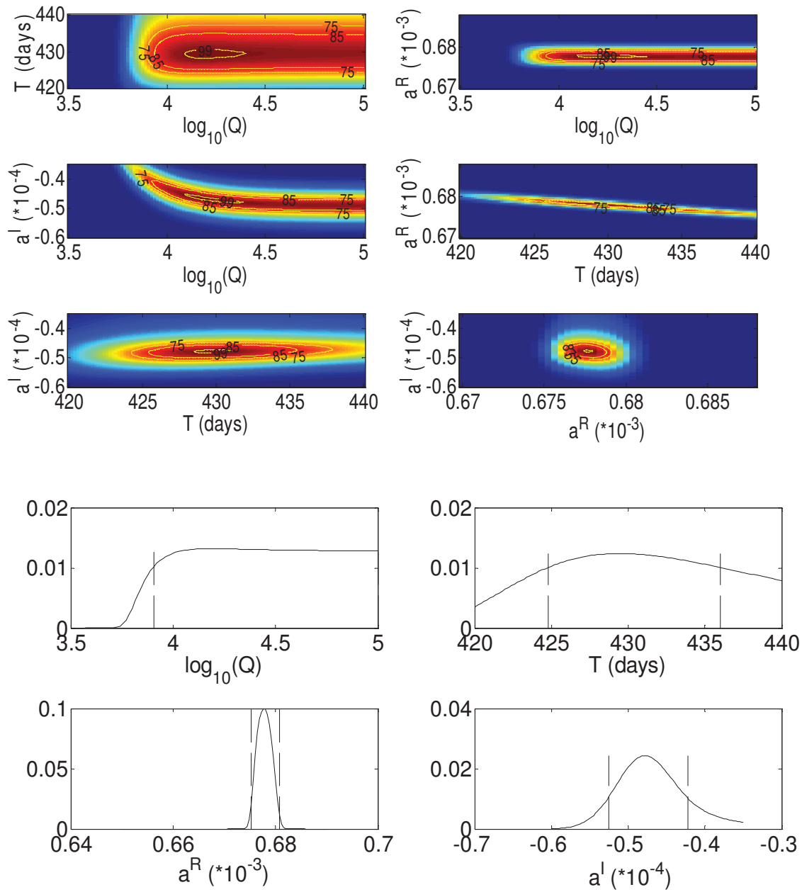
Fig. 6.11: Joint and marginal probability density functions for the FCN parameters ( \mathbf{a}_r , \mathbf{a}_i , \mathbf{T} and \mathbf{x} ) estimated from 18 years of SG C026 data using the Bayesian method. Vertical dotted lines indicate the 90% confidence intervals.
