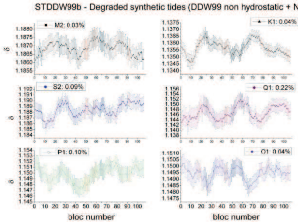
Fig. A.4: Time variability of the delta factors for a synthetic tidal model (DDW99+NAO99) at J9 showing the pre-processing effect.
