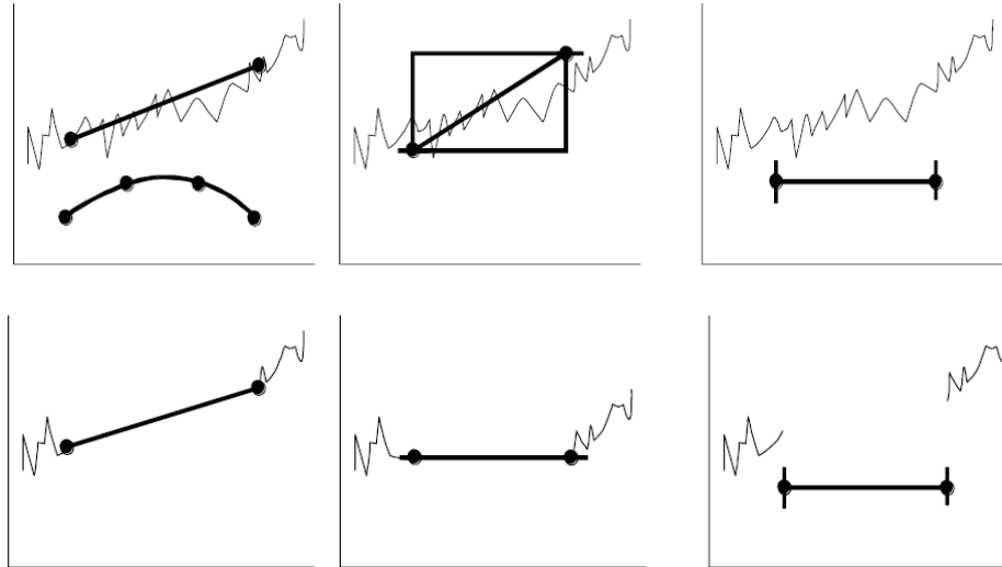
Fig. 2.3.3: Graphical representation of the different correctors offer by TSOFTE, in unapplied state (upper) and in applied state (bottom). Left: linear and cubic interpolations; middle: step; right: gap (from TSOFTE manual).
