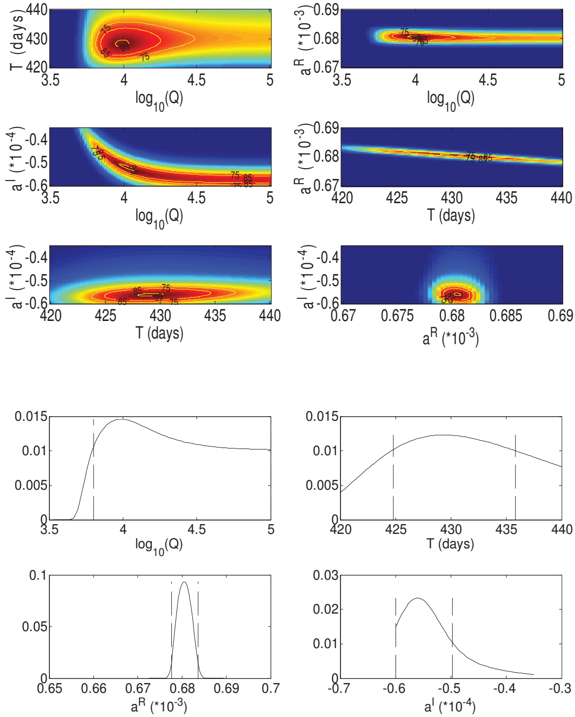
Fig. 6.13: Joint and marginal probability density functions for the FCN parameters ( a^r , a^i , T and x ) estimated from stacking 7 European SG (Bad-Homburg, J9 (Strasbourg), Moxa, Membach, Medicina, Strasbourg, Vienna and Wettzell) records using the Bayesian method. Vertical dotted lines indicate the 90% confidence intervals.
