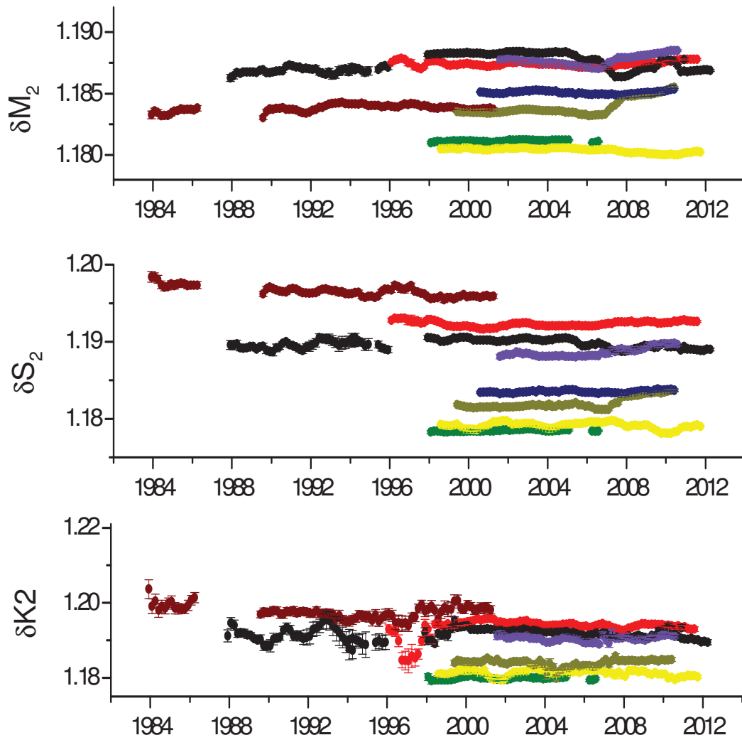
Fig. 4.18: Temporal variations of the tidal amplitude factors for the main semidiurnal waves ( M_2 , S_2 , K_2 ), obtained from the tidal analysis using ETERNA 3.4 software on yearly segments shifted month by month of 8 European SGs, with no ocean loading correction applied. The resulting tidal parameters are associated to the central epoch of the analyzed interval.
