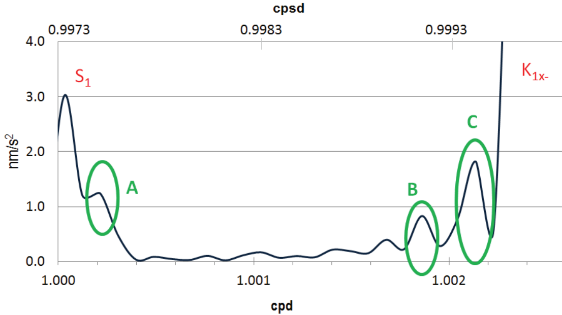
Fig. 6.15: Amplitude spectra of the complete (9760 days, 26.7 years) SG record (T005 + C026) in Strasbourg J9 Observatory between S1 and K1x- waves.
