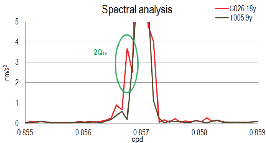
Fig. E.1: Spectral analyses in the diurnal frequency band of the 18 years series of the SG C026 in red, and of the merged 27 year series recorded both by T005 and C026 in black, at Strasbourg J9 Observatory.
