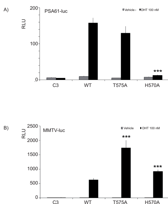
Figure S5. Luciferase reporter assay for AR-WT, AR-T575A and AR-H570A. The H570A mutation orientates androgen receptor transactivation towards the non-specific responsive promoter. LNCaP cells were cotransfected with AR DBD-WT or the indicated mutant expression plasmid together with PSA61-Luc (A) or MMTV-luc (B) firefly luciferase construct and pGL4.70[hRLuc] (Renilla) for transfection control. Cells were then treated with 100nM DHT or vehicle in serum-free medium for 48 hours. Luminescence (relative light units) was normalized to the Renilla luciferase expression from the pGL4.70[hRLuc]. P values of less than 0.05 were considered significant (***)
