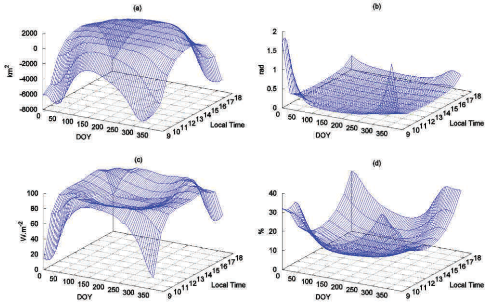
Figure 5.9: Hourly and daily variation of differences between sub-pixel and pixel level corrections for: (a) Shadow binary factor, in \text{km}^2 of lightened area; (b) ratio between incidence and zenith solar angle in radian; (c) Total irradiance values in \text{W.m}^{-2} ; (d) Total irradiance normalized (Equation 5.13) values in %
