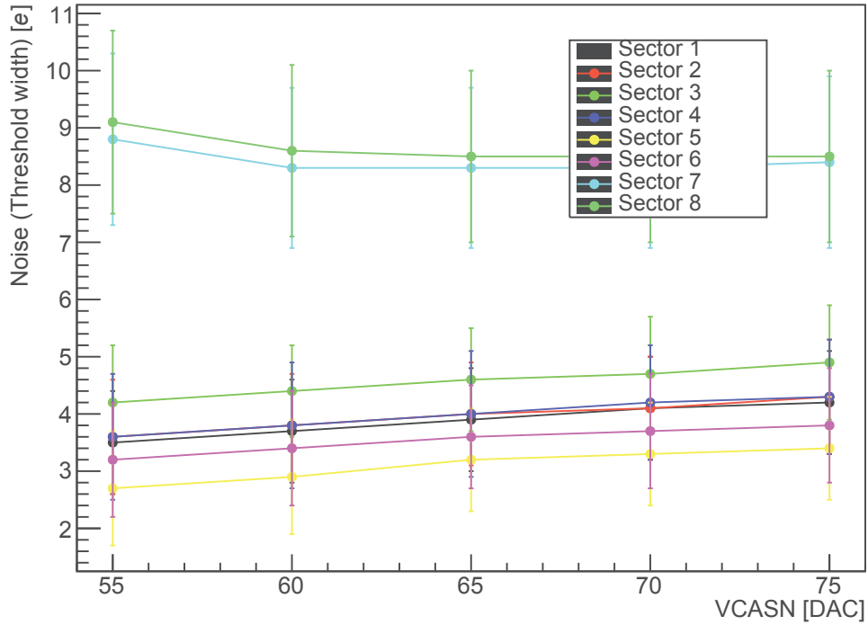
Figure 3.10: Mean threshold width as a function of VCASN for ITHR = 60 for each of the 8 sectors of the pALPIDEfs-3 chip.
