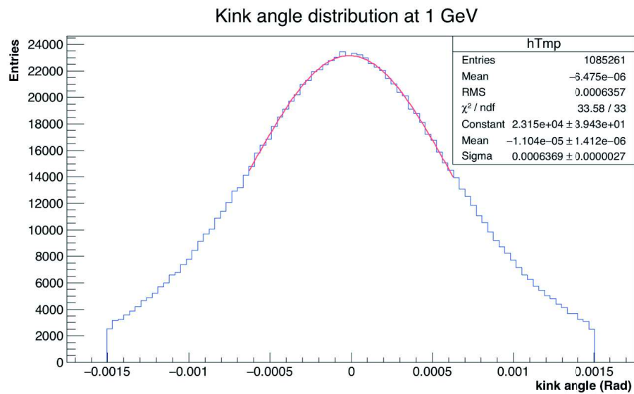
Figure 7.13 – Distribution of the kink angle \theta_0 given by GBL for an energy of 1 GeV without any fiducial cut.
