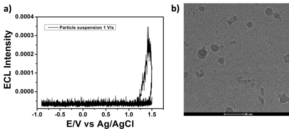
Figure 2.13. a ) ECL emission of Pt-Amide particles suspension solution recorded during a cyclic voltammetry at scan rate 1 \text{ V s}^{-1} in PBS solution upon addition of 10 mM TPrA; b ) TEM image of particles suspension (scale bar = 50 nm).
