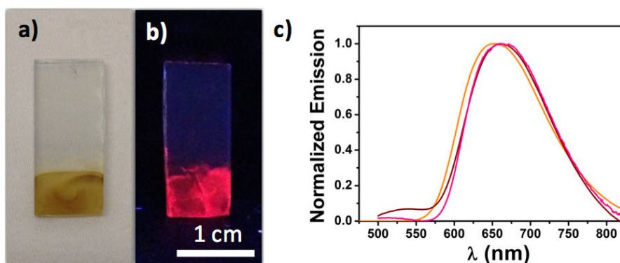
Figure 3.8. a) Electropolymerised FTO electrode after 15 scans, b) under UV lamp, c) emission spectra of 10^{-5} M Ir(pphen) 2 (mVbpy) in CH 3 CN (orange trace), poly-Ir on FTO electrode after 15 scans (brown trace) and poly-Ir on FTO electrode after 50 scans (pink trace). \lambda_{exc} = 450 nm.
