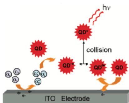
Figure 1.13. Anodic ECL mechanism of QDs. Reprinted from reference (83).
