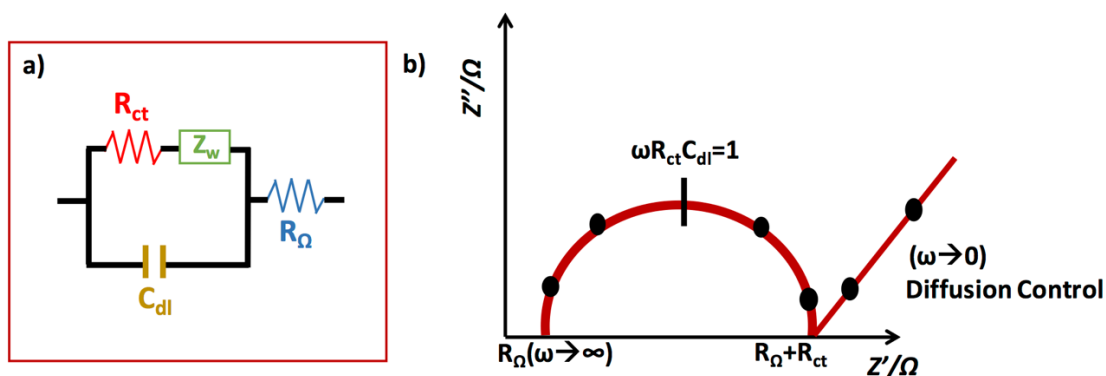
Figure 6.3. a) Randles equivalent circuit for a simple electrochemical system; b) Nyquist plot arising from the Randles circuit.
