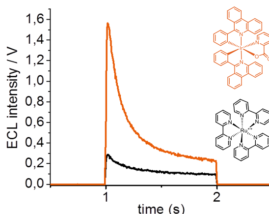
Figure 1.10. ECL response during time of [\text{Ir}(\text{pphent})(\text{pic})] and \text{Ru}(\text{bpy})_3^{2+} under 1s potentiostatic impulse at + 1.4 V vs Ag/AgCl, reported in reference (54).
