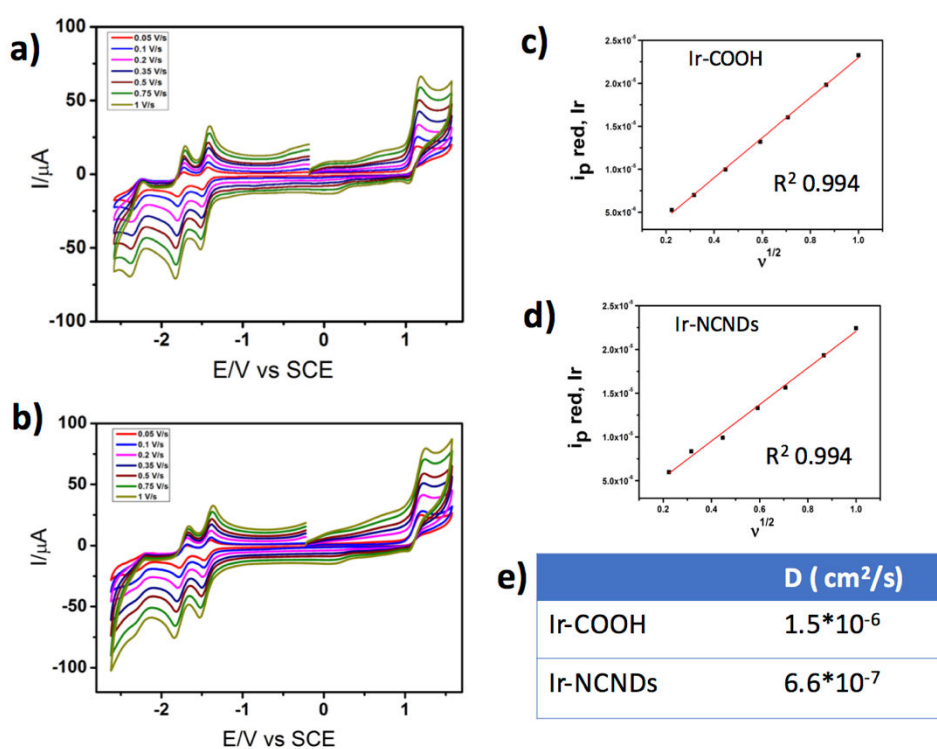
Figure 5.12. a) CVs of Ir-COOH, b) CVs of Ir-NCNDs at the same concentration of chromophores (1 mM) in 0.1 M TBAPF 6 DMF solution and GC (1 mm) as working electrode. Scan rate from 0.05 V s -1 to 1 V s -1 ; i_p vs v^{1/2} of c) CVs of Ir-COOH and d) CVs of Ir-NCNDs. e) table reporting the diffusion coefficients (D, cm 2 /s) calculated by using Randles-Sevcik equation for Ir-COOH and Ir-NCNDs.
