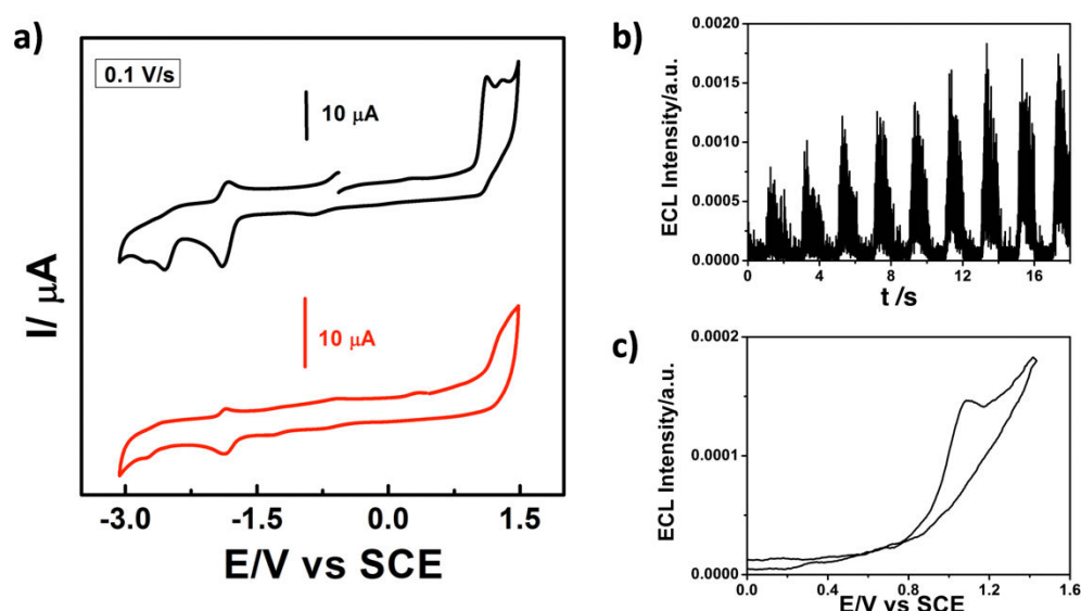
Figure 2.8. a) Cyclic voltammograms of 1 mM (black trace) and 0.1 mM (red trace) Pt-Amide in 0.1 M \text{TBAPF}_6 \text{CH}_3\text{CN} solution at GC electrode. Scan rate 0.1 \text{ V s}^{-1} . SCE as reference electrode and Pt wire as counter electrode; b) ECL emission of 1 mM Pt-Amide in 0.1 M \text{TBAPF}_6 \text{CH}_3\text{CN} solution generated by ion annihilation at GC electrode with pulsing (1 s) between 2 nd oxidation and 1 st reduction peak potentials of the complex; c) ECL emission of 1 mM Pt-Amide recorded during a cyclic voltammetry at scan rate 0.05 \text{ V s}^{-1} in 0.1 M \text{TBAPF}_6 \text{CH}_3\text{CN} solution with 1 mM TPrA as co-reactant.
