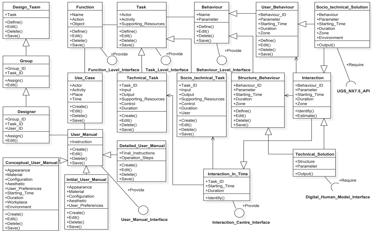
Figure 4.6. Class diagram of IDC module
