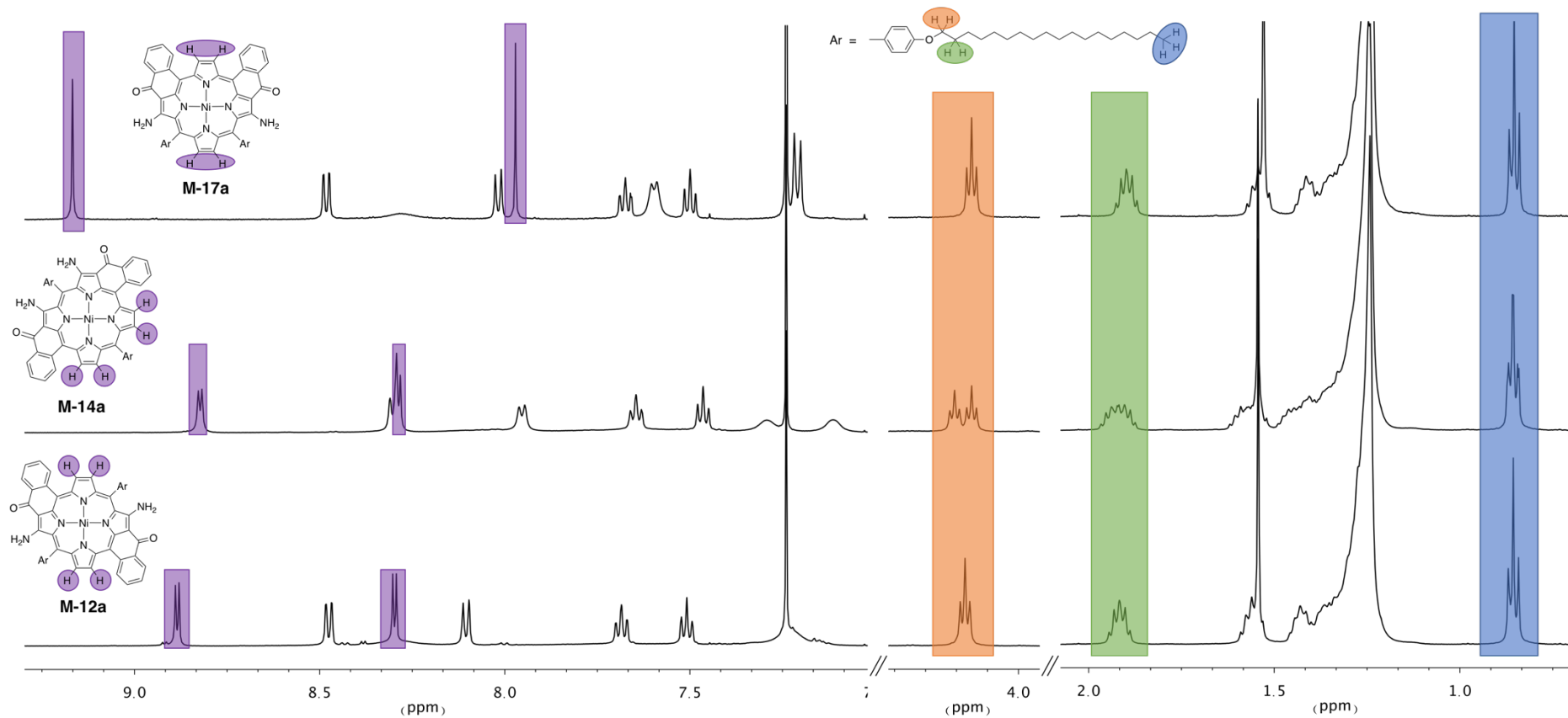
Figure 3. Spectres RMN ^1\text{H} de M-12a , M-14a et M-17a , Ar = \text{Ph-OC}_{18}\text{H}_{37}
