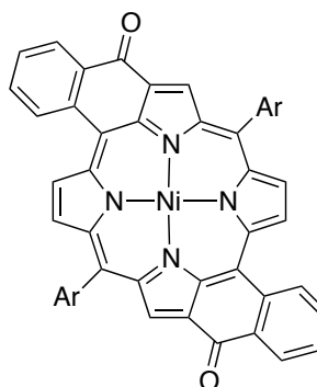
5,15-bi-ketone2 porphyrin
