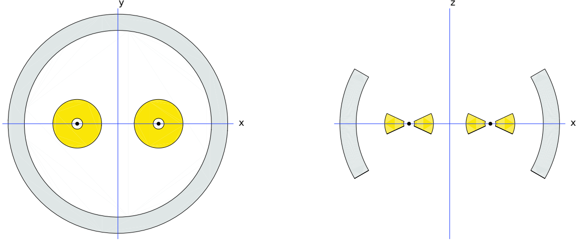
Figure 6.5: Cartoon illustrating equatorial scattering region. Left figure shows the face-on view, while on the right the same geometry is shown when viewed edge-on. An example is shown for the case with the two BLRs being separated. The BLRs are shown in yellow. Scattering region is denoted in grey. Credits: Savić et al. (2019) .
