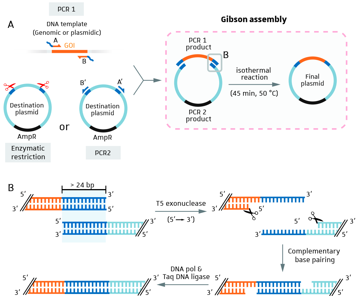
Figure MM-3: Overview of assembling DNA fragments by the isoT cloning method. (A) The gene of interest (GOI) is amplified with primers A and B that contain isoT overhangs (dark blue) and yields a linear DNA fragment flanked by homologous extremities present in the destination plasmid. The destination plasmid is amplified with primers A' and B' or cleaved by restriction enzymes, so that 5' and 3' extremities of the linearized plasmid overlap with the 3' and 5' extremities of the amplified GOI, respectively. The extremities of both linearized fragments are assembled by the isothermal Gibson assembly method (isoT), detailed in B, and results in a final plasmid in which the GOI is cloned. (B) The 3' and 5' extremities of the linearized GOI and the destination plasmid, respectively, are colored in dark blue and the homologous overlap is indicated by the transparent blue rectangle. The “chaw-back” step is achieved during the first step of isoT assembly by the T5 exonuclease which releases 3' single stranded extremities, thereby enabling complementary base-pairing. The remaining gaps are filled in and sealed through the combined activities of a thermostable DNA pol and the Taq DNA ligase. All these steps are combined in a single assay that leads to the fact that the isoT assembly can be considered as a one-step reaction performed at 50°C for 25 min.
