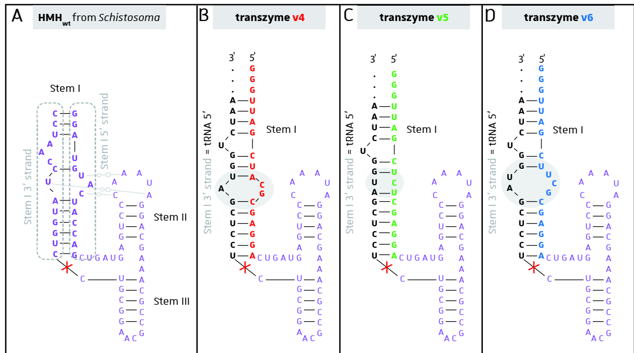
Figure RT-4: Secondary structure of the HMH wt ribozyme and covariance model folds of HMH wt -tRNA Asp Afm transzymes used in this study. (A) The wt sequence of the HMH ribozyme is in purple and stem I's (substrate stem) 5' and 3' strands are annotated. X indicates the cleavage site. HMH wt -tRNA Asp Afm transzymes v4 (B), v5 (C) and v6 (D) were designed using HMH wt as background. During the design, the 5' sequence of the tRNA (in black and bold) was fused to the HMHwt and the 5' strand (red for v4, green for v5 and blue for v6) of the substrate stem was adapted to obtain partial complementarity so that essential unpaired structures (bulges; see text) are conserved. In this way the 5' sequence of the tRNA dictates the sequence of the 3' strand of the expected ribozyme stem I.
