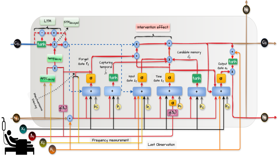
Figure 6.2: AMITA Unit on analyzing patient’s EHR records. Sketch red arrows correspond to the modifications compared to LSTM Unit. Shade blue boxes indicate networks and shade blue circles denote point-wise operators.
